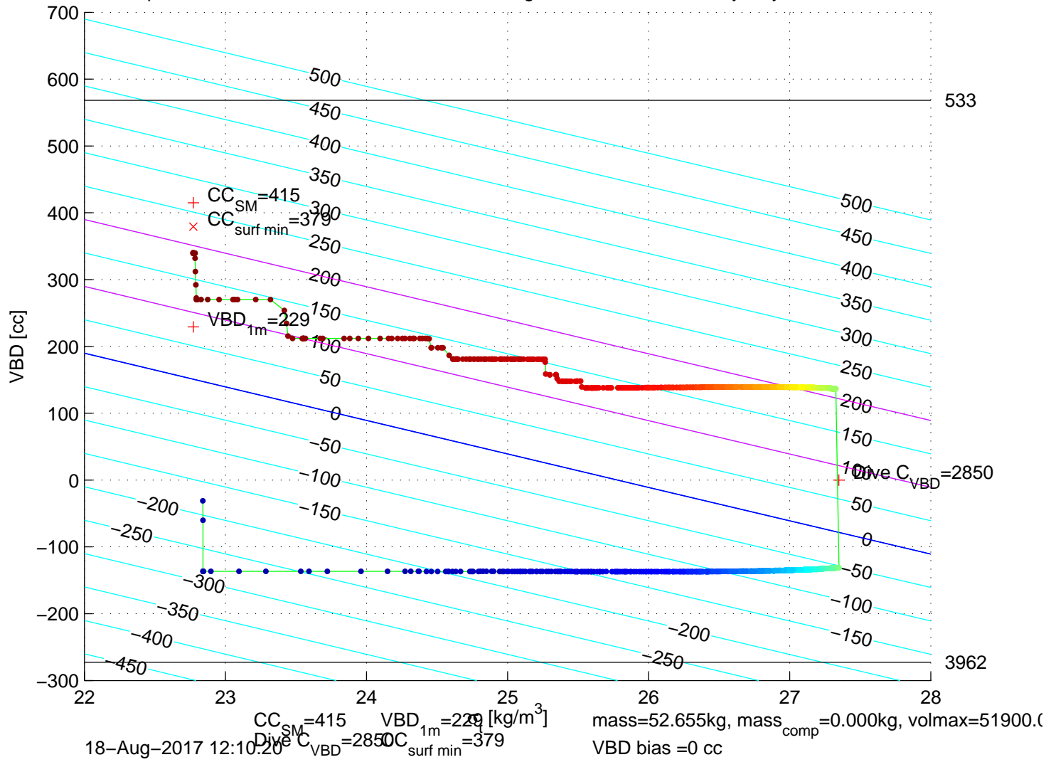
p6350217: SG635 Mission 7 Jul 2017 18-Aug-2017 11:52:09Z – buoyancy contoured
