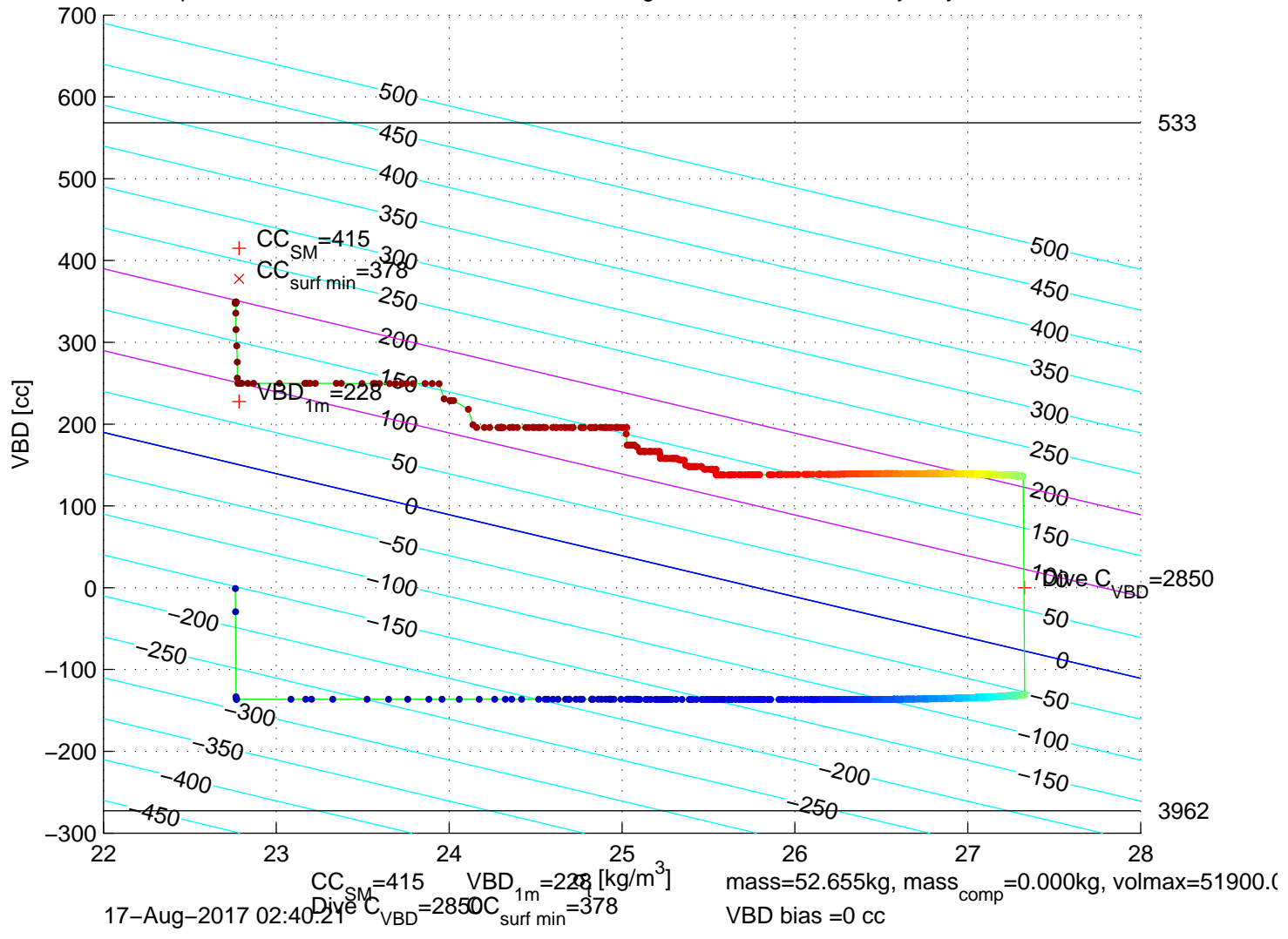
p6350209: SG635 Mission 7 Jul 2017 17-Aug-2017 02:27:44Z – buoyancy contoured
