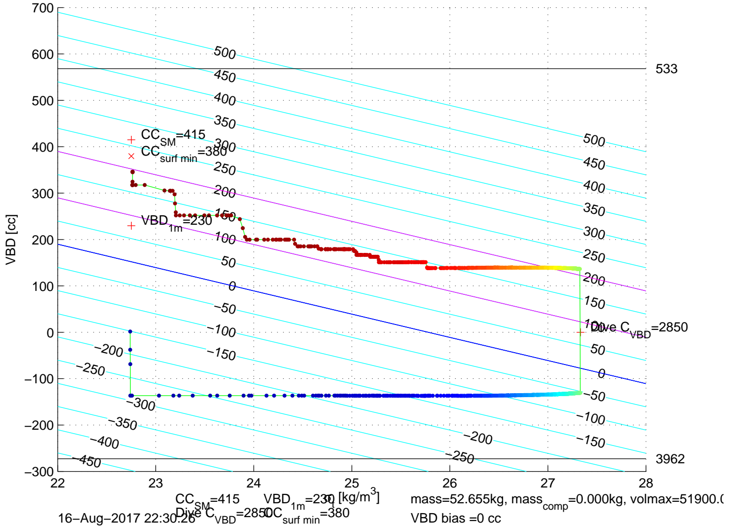
p6350208: SG635 Mission 7 Jul 2017 16–Aug–2017 22:19:21Z – buoyancy contoured
