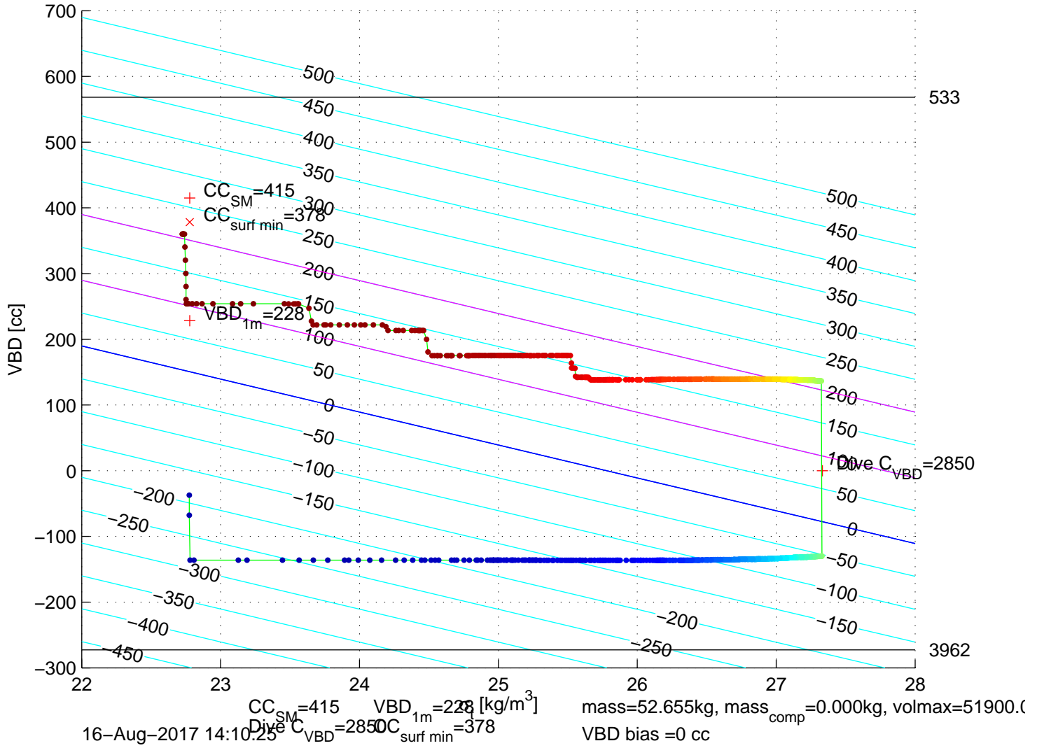
p6350206: SG635 Mission 7 Jul 2017 16–Aug–2017 13:55:26Z – buoyancy contoured
