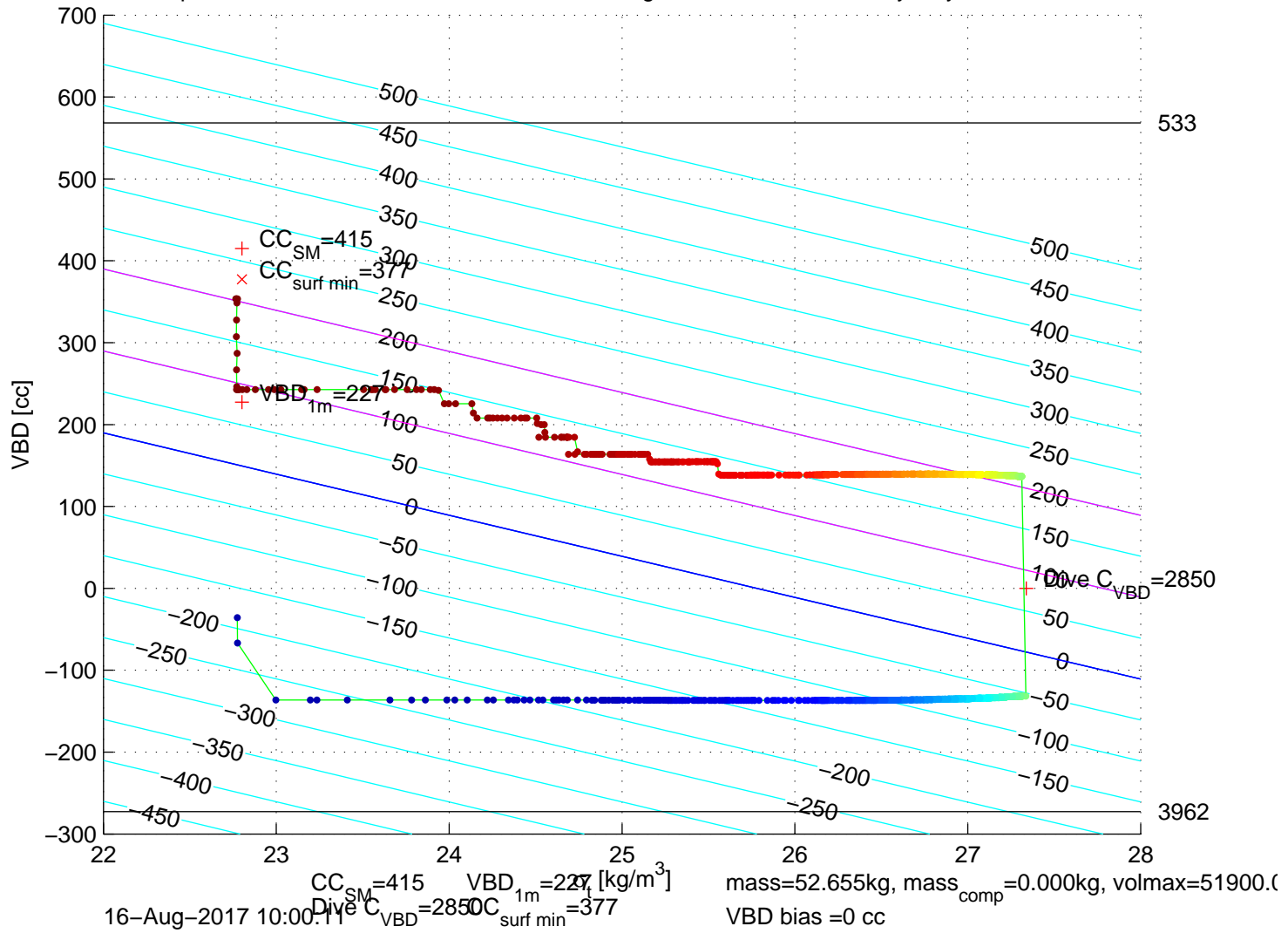
p6350205: SG635 Mission 7 Jul 2017 16-Aug-2017 09:44:16Z – buoyancy contoured
