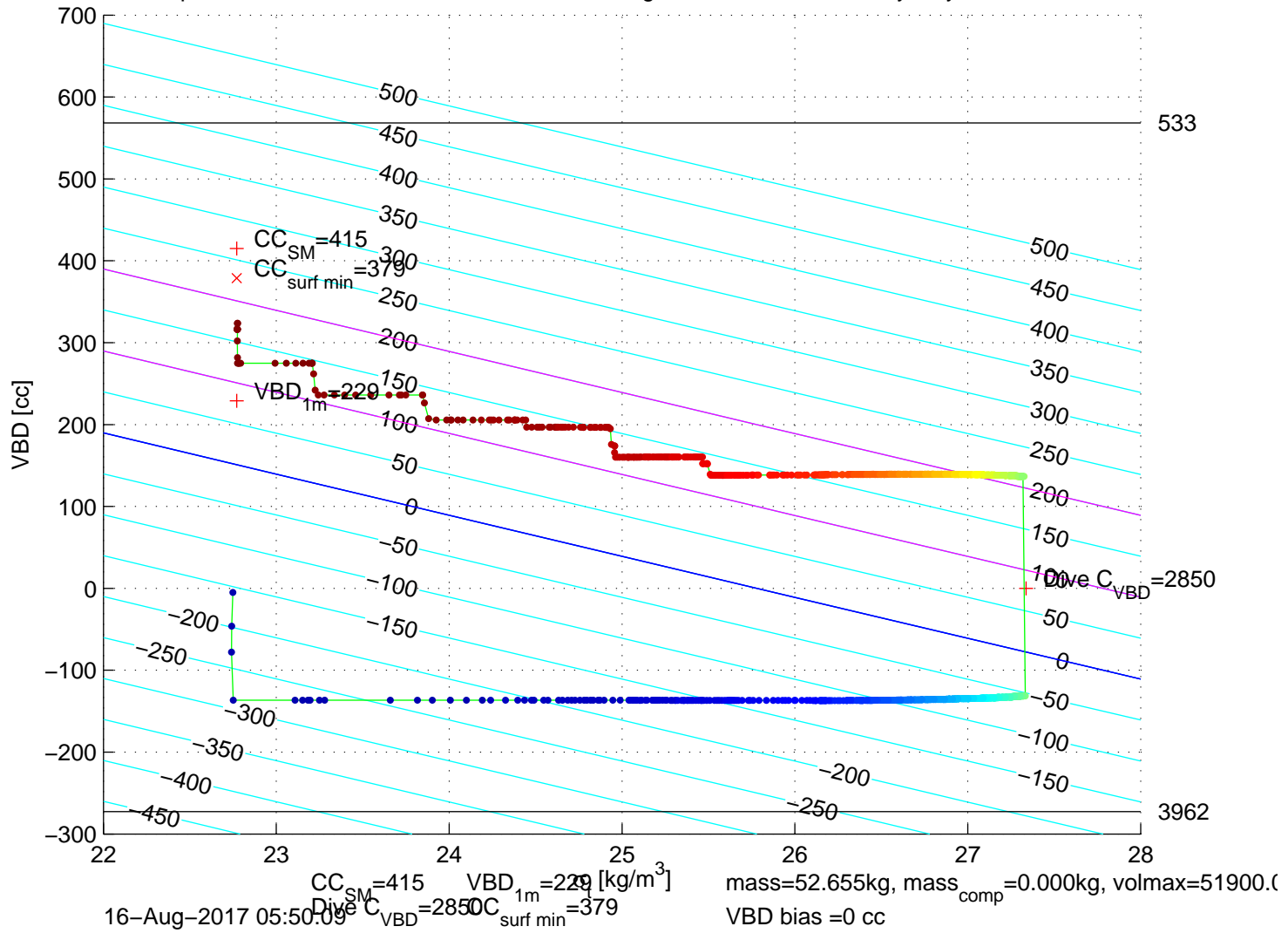
p6350204: SG635 Mission 7 Jul 2017 16-Aug-2017 05:40:27Z – buoyancy contoured
