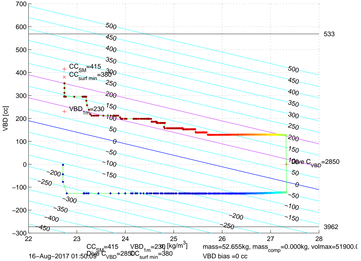
p6350203: SG635 Mission 7 Jul 2017 16-Aug-2017 01:25:16Z – buoyancy contoured
