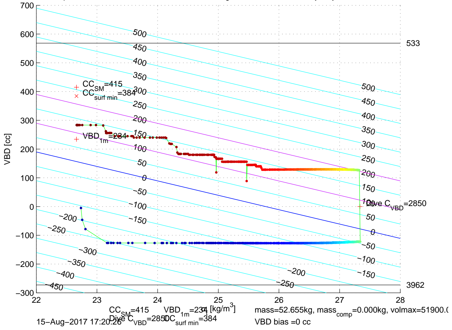
p6350201: SG635 Mission 7 Jul 2017 15–Aug–2017 17:03:55Z – buoyancy contoured
