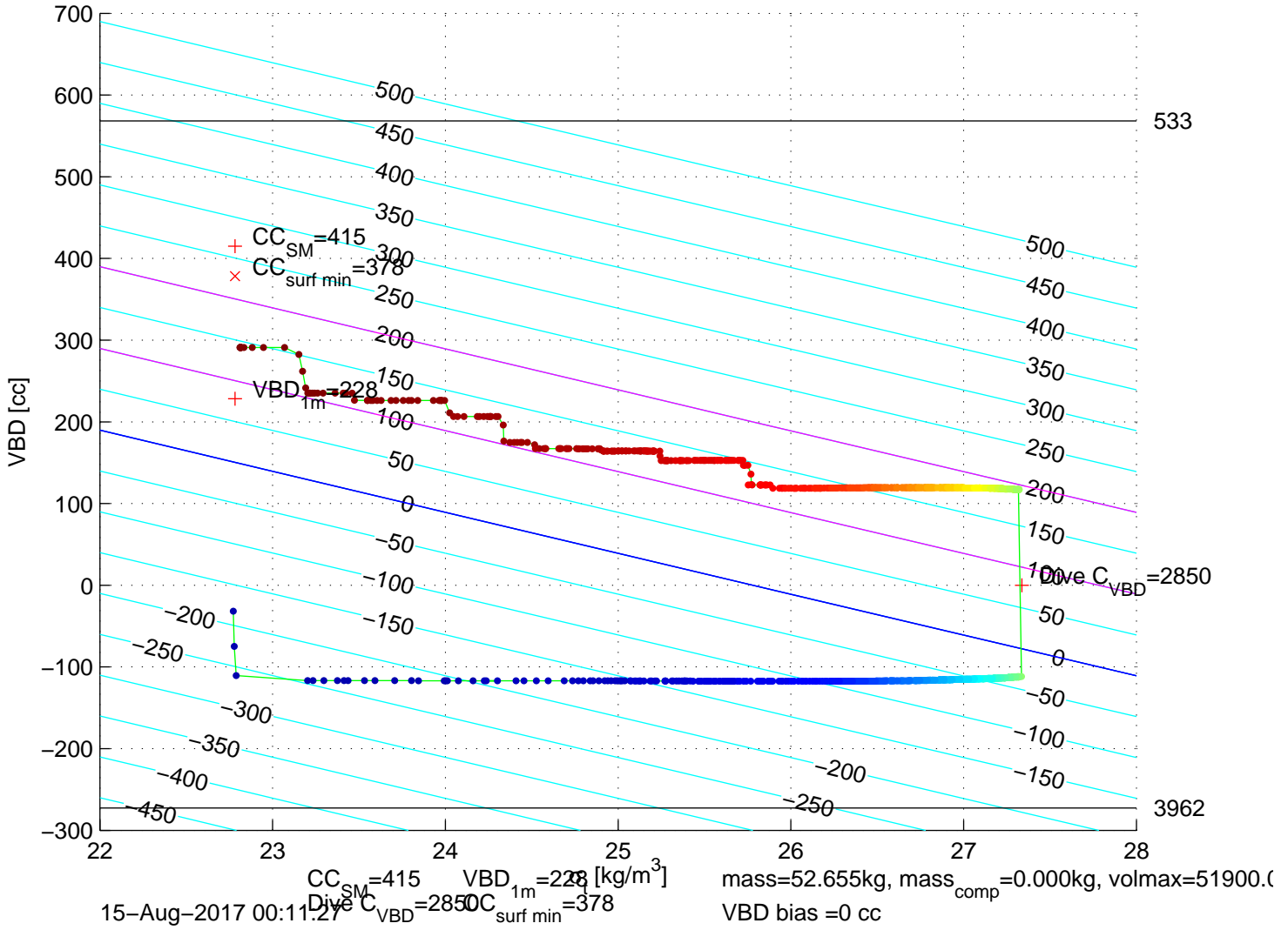
p6350197: SG635 Mission 7 Jul 2017 14-Aug-2017 23:47:07Z – buoyancy contoured
