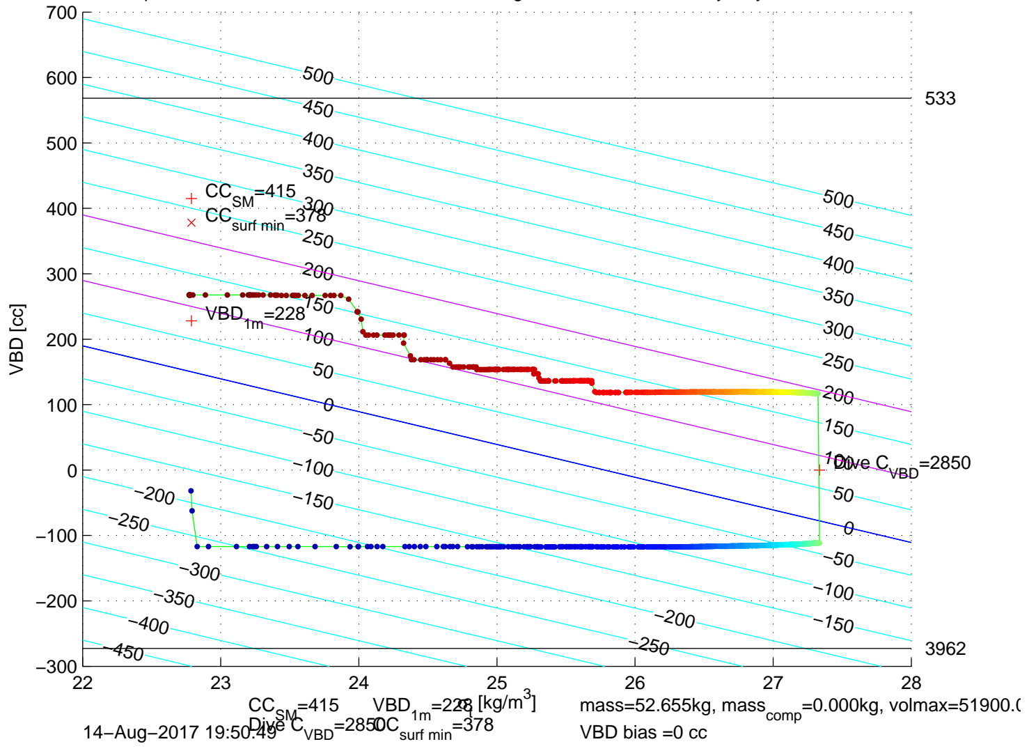
p6350196: SG635 Mission 7 Jul 2017 14-Aug-2017 19:27:40Z – buoyancy contoured
