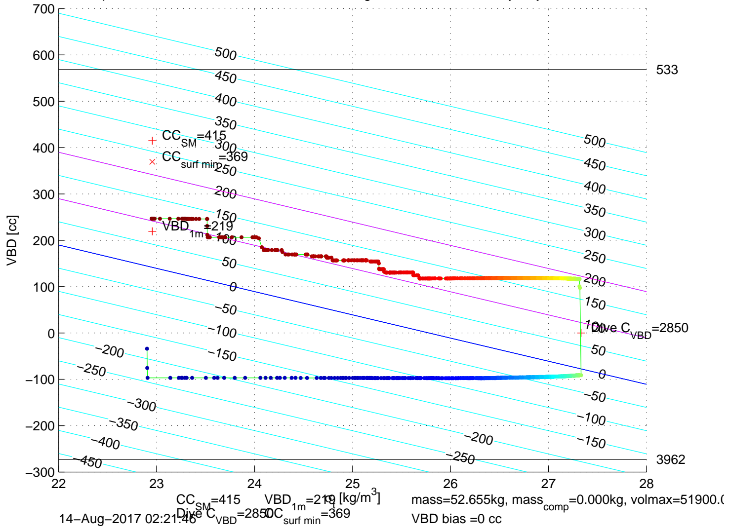
p6350192: SG635 Mission 7 Jul 2017 14-Aug-2017 01:46:26Z – buoyancy contoured
