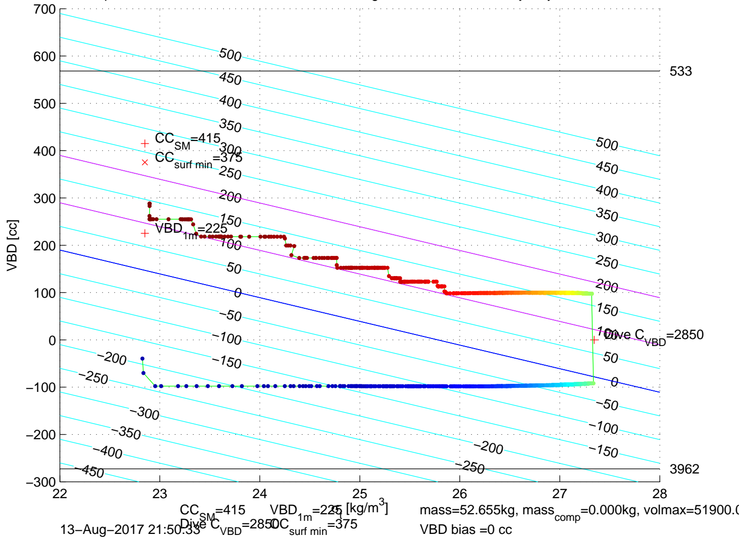
p6350191: SG635 Mission 7 Jul 2017 13-Aug-2017 21:10:54Z – buoyancy contoured
