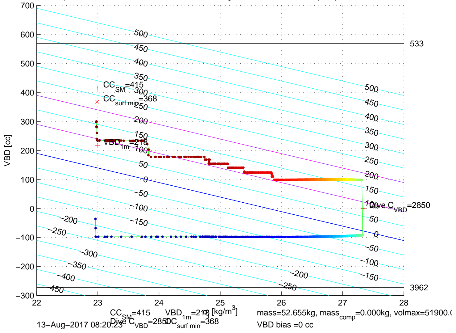
p6350188: SG635 Mission 7 Jul 2017 13-Aug-2017 07:42:55Z – buoyancy contoured
