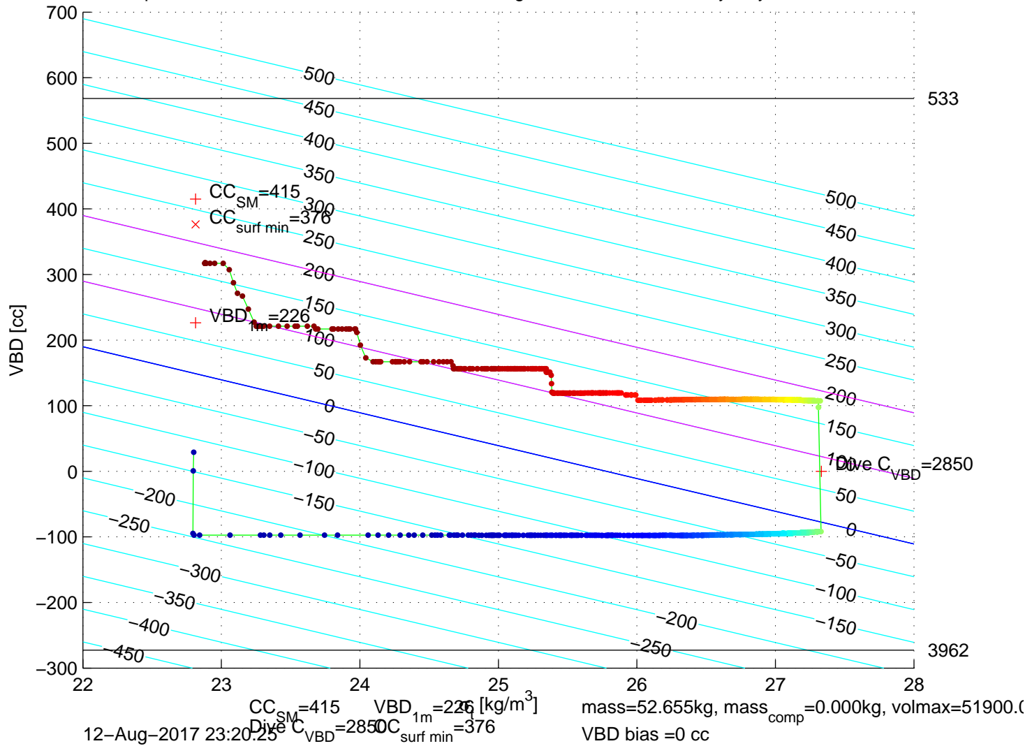
p6350186: SG635 Mission 7 Jul 2017 12-Aug-2017 22:53:18Z – buoyancy contoured
