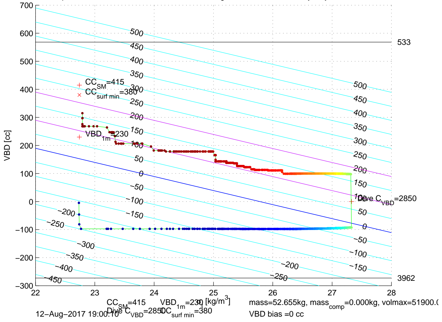
p6350185: SG635 Mission 7 Jul 2017 12-Aug-2017 18:18:19Z – buoyancy contoured
