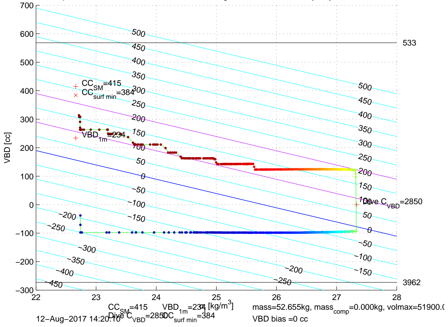
p6350184: SG635 Mission 7 Jul 2017 12–Aug–2017 14:05:35Z – buoyancy contoured
