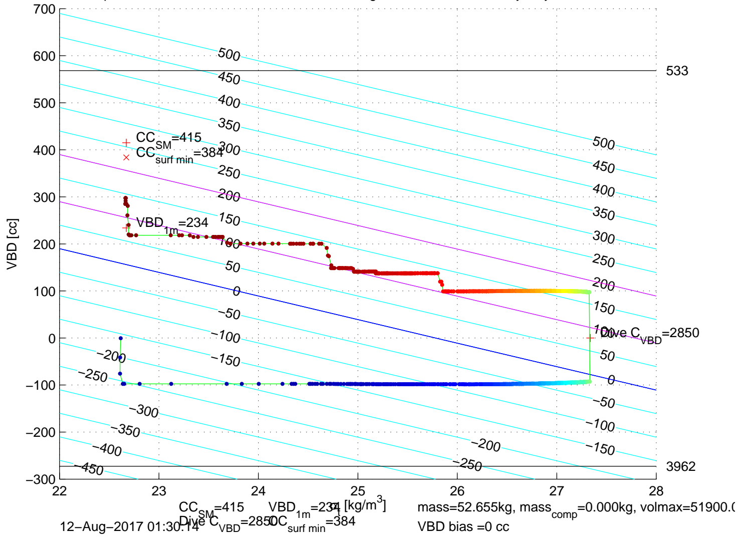
p6350181: SG635 Mission 7 Jul 2017 12-Aug-2017 00:52:55Z – buoyancy contoured
