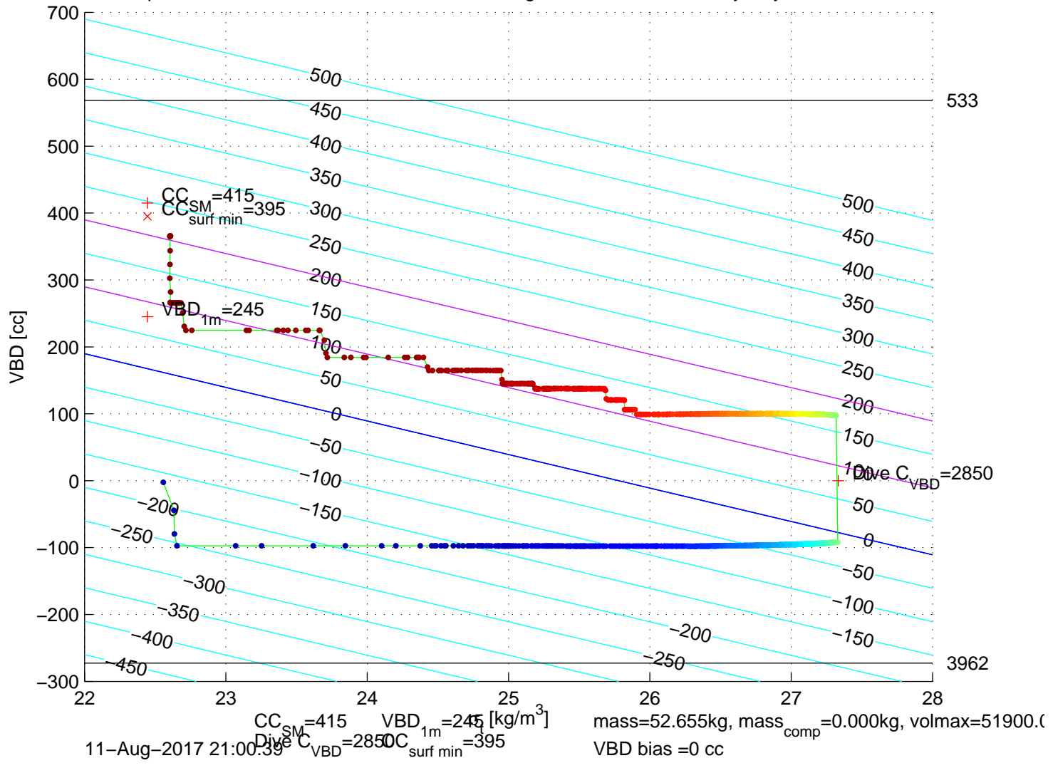
p6350180: SG635 Mission 7 Jul 2017 11–Aug–2017 20:24:28Z – buoyancy contoured
