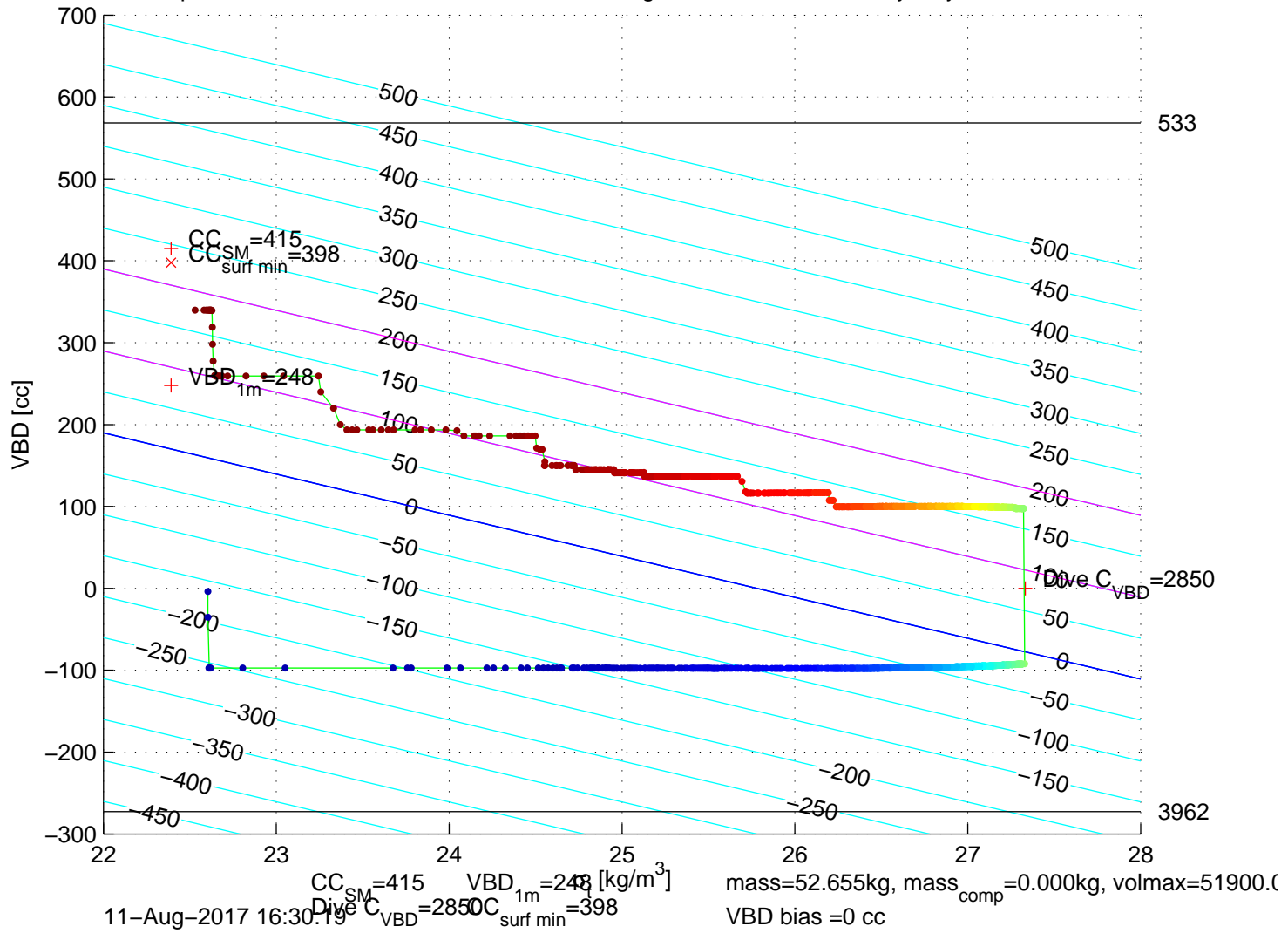
p6350179: SG635 Mission 7 Jul 2017 11-Aug-2017 15:55:33Z – buoyancy contoured
