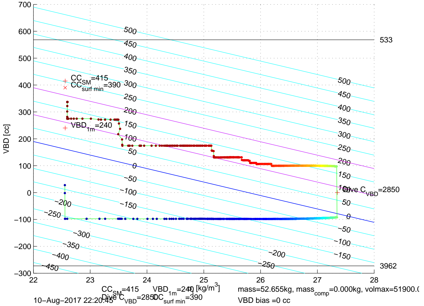
p6350175: SG635 Mission 7 Jul 2017 10–Aug–2017 21:44:36Z – buoyancy contoured
