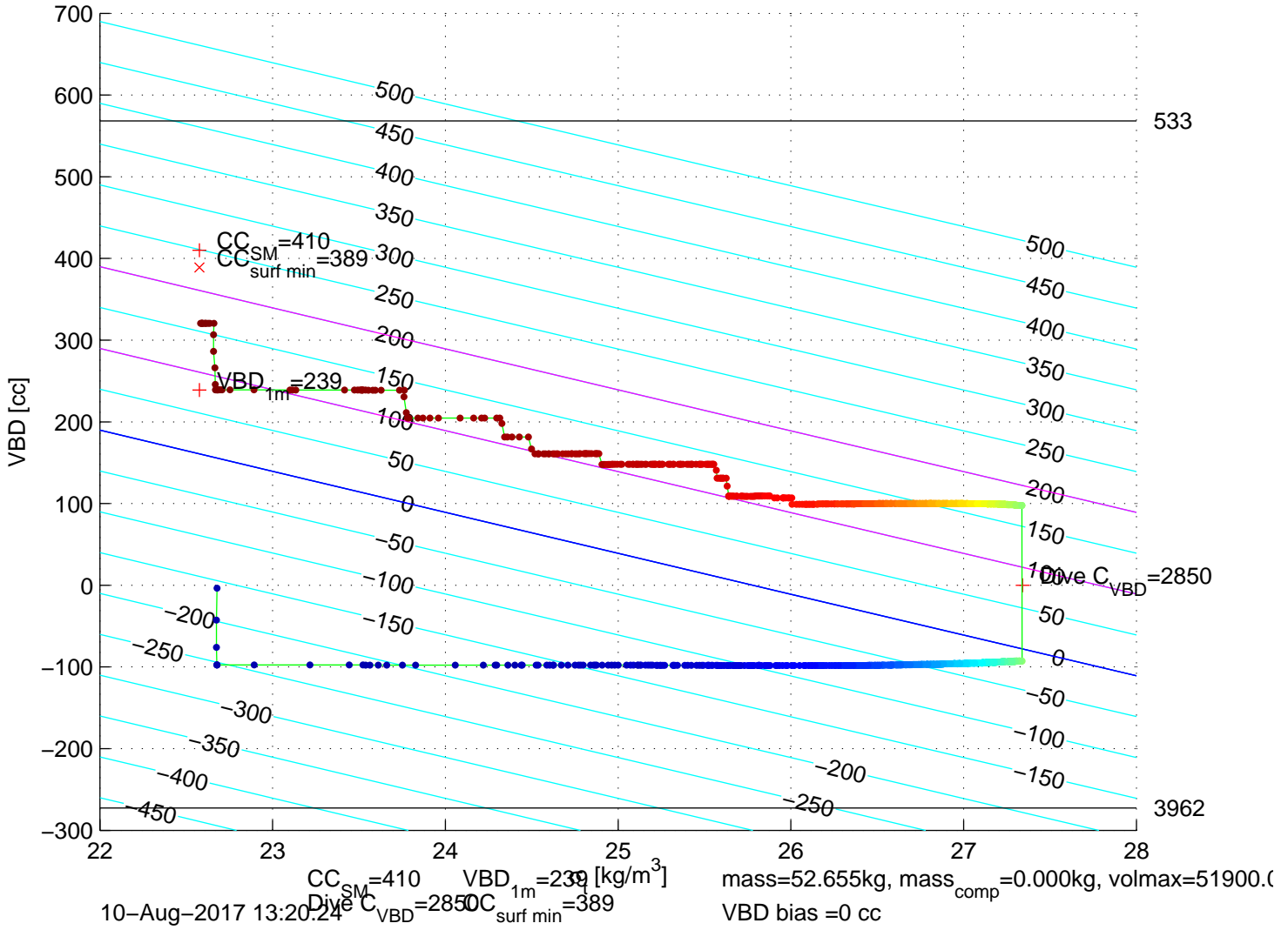
p6350173: SG635 Mission 7 Jul 2017 10-Aug-2017 12:43:33Z – buoyancy contoured
