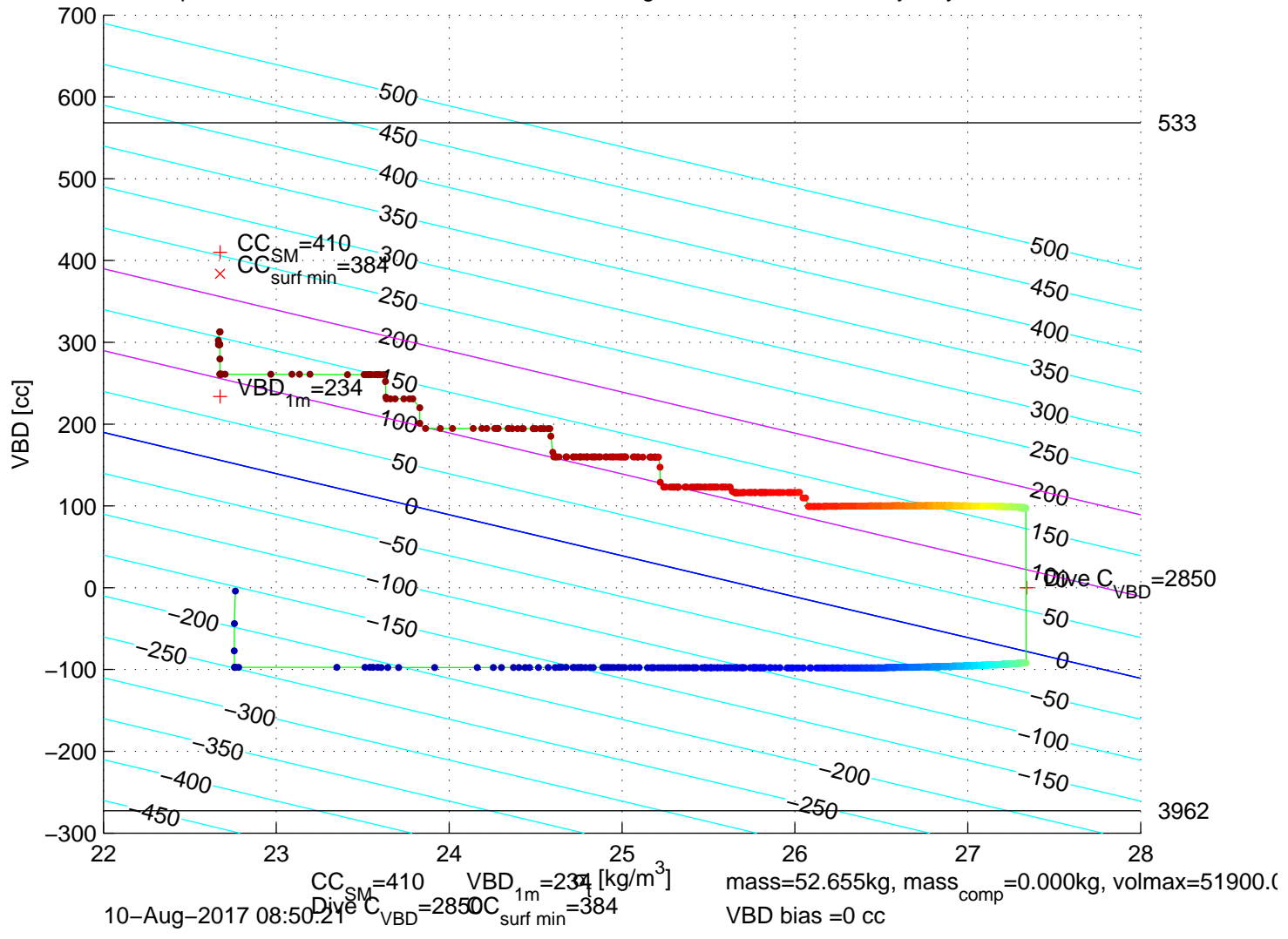
p6350172: SG635 Mission 7 Jul 2017 10–Aug–2017 08:12:20Z – buoyancy contoured
