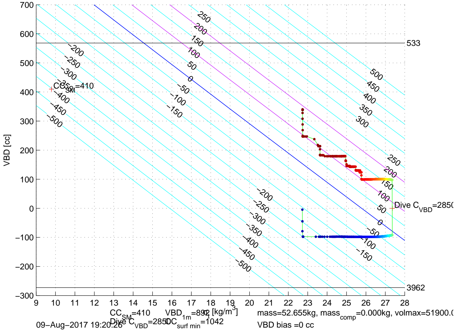
p6350169: SG635 Mission 7 Jul 2017 09–Aug–2017 18:42:58Z – buoyancy contoured
