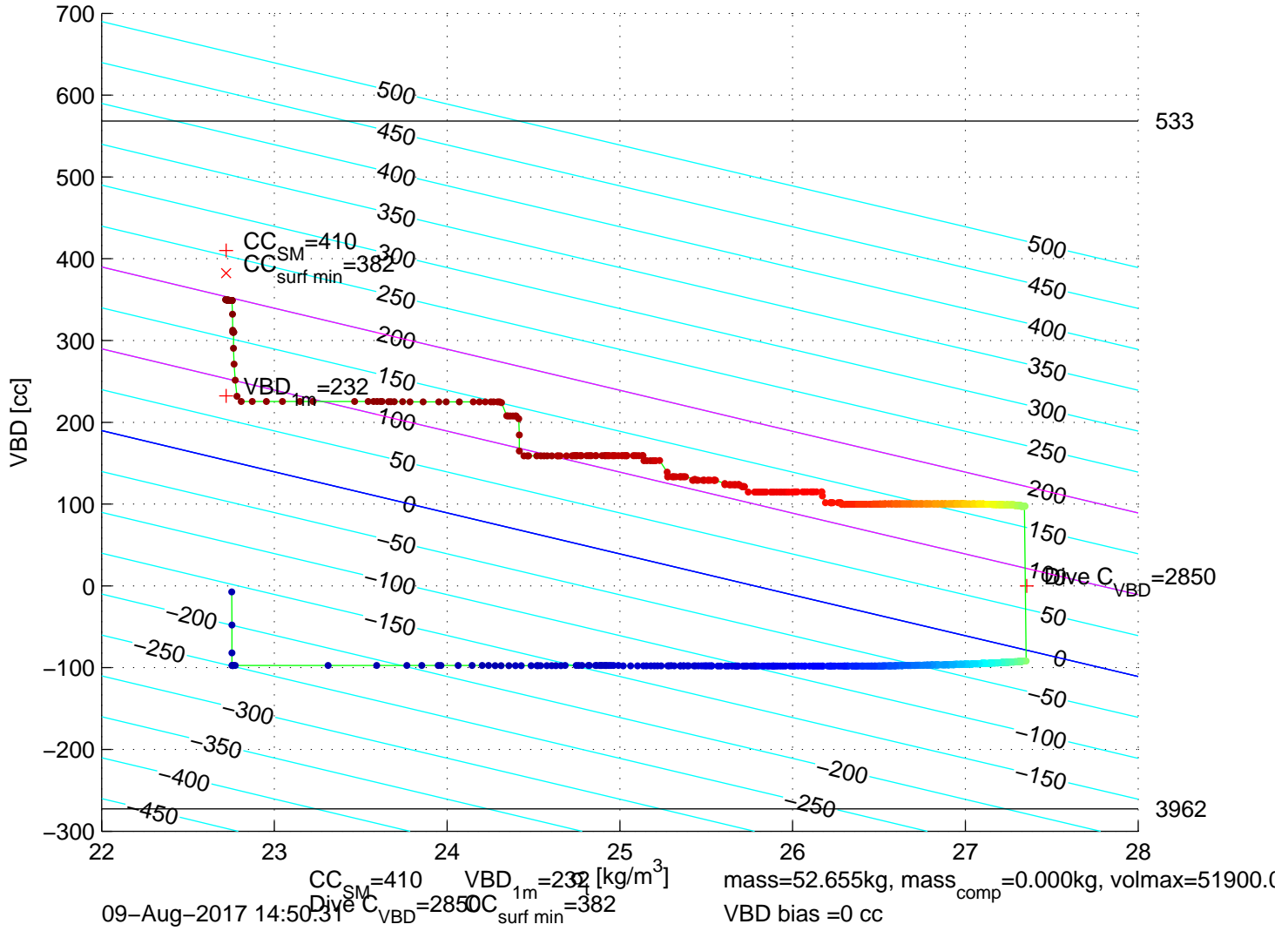
p6350168: SG635 Mission 7 Jul 2017 09–Aug–2017 14:13:13Z – buoyancy contoured
