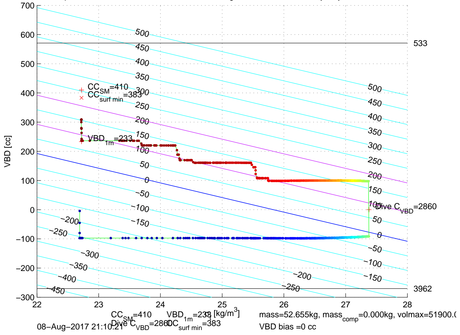
p6350164: SG635 Mission 7 Jul 2017 08-Aug-2017 20:37:38Z – buoyancy contoured
