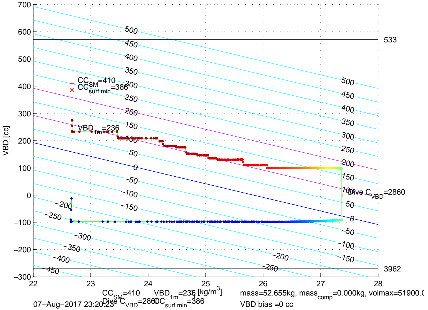
p6350159: SG635 Mission 7 Jul 2017 07-Aug-2017 22:43:21Z - buoyancy contoured
