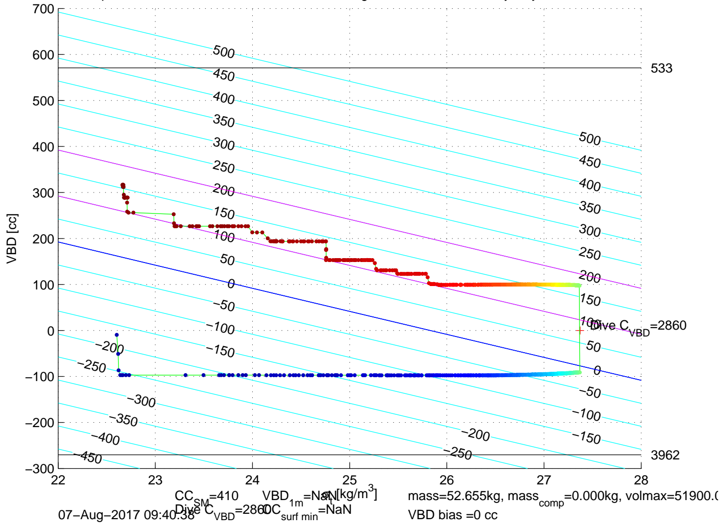
p6350156: SG635 Mission 7 Jul 2017 07–Aug–2017 09:07:36Z – buoyancy contoured
