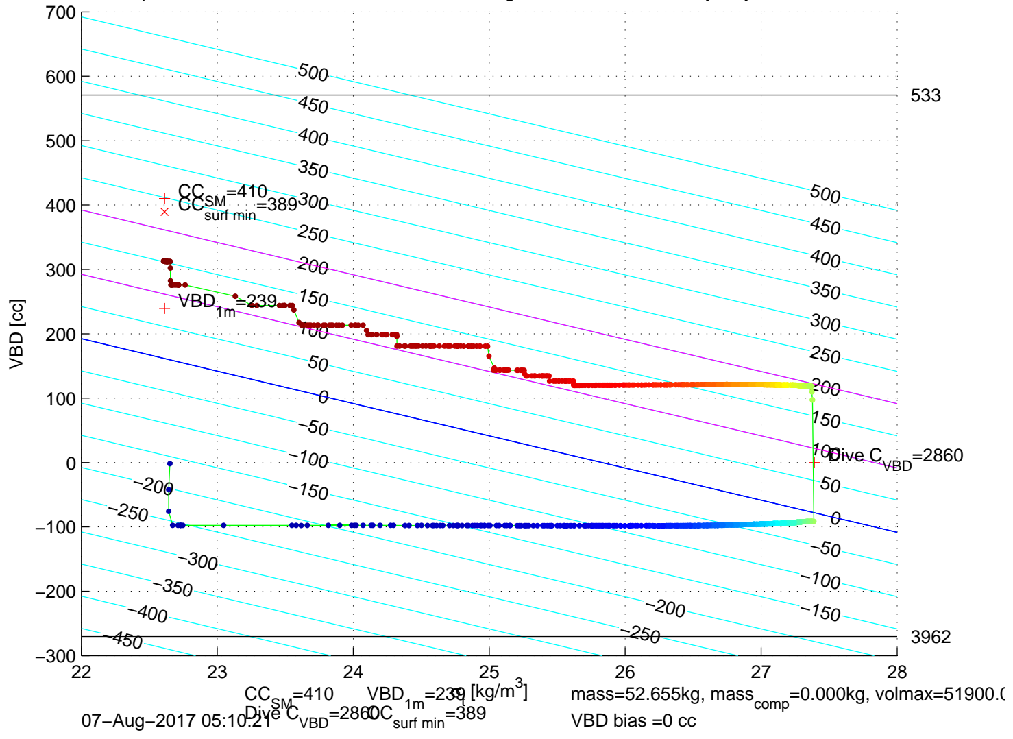
p6350155: SG635 Mission 7 Jul 2017 07–Aug–2017 04:47:17Z – buoyancy contoured
