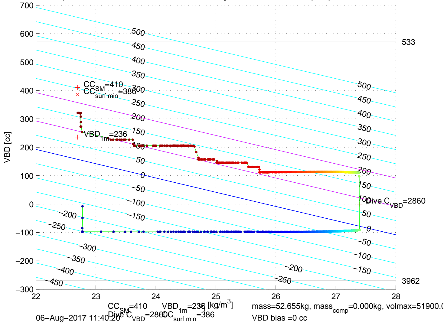
p6350151: SG635 Mission 7 Jul 2017 06–Aug–2017 11:12:06Z – buoyancy contoured
