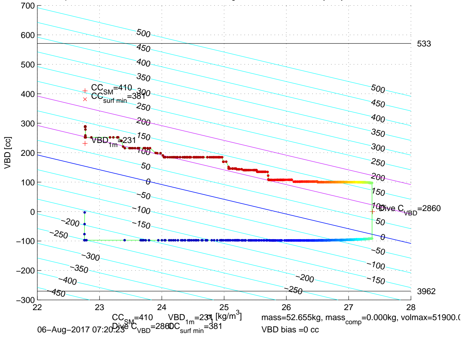
p6350150: SG635 Mission 7 Jul 2017 06–Aug–2017 06:41:38Z – buoyancy contoured
