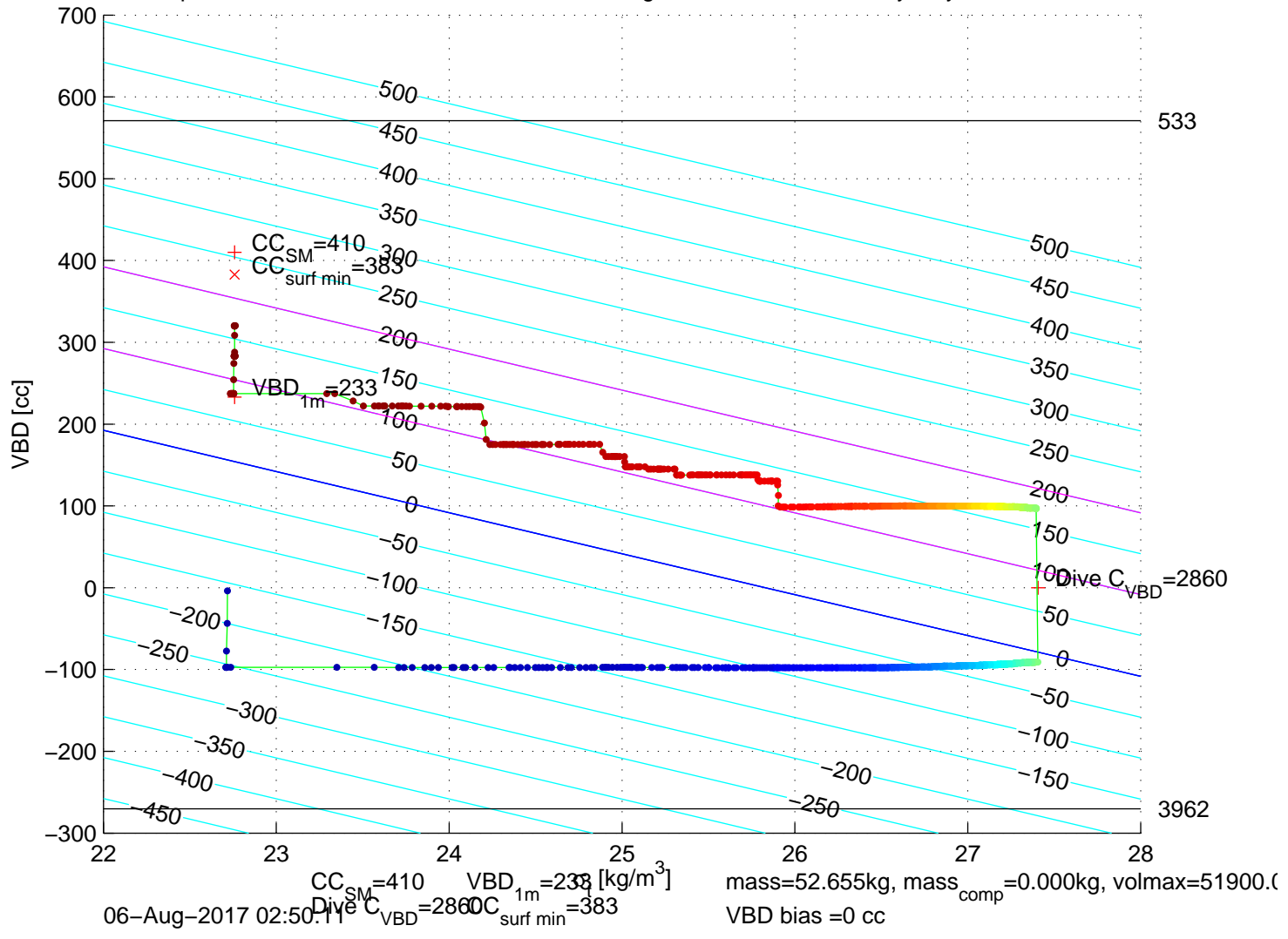
p6350149: SG635 Mission 7 Jul 2017 06–Aug–2017 02:08:47Z – buoyancy contoured
