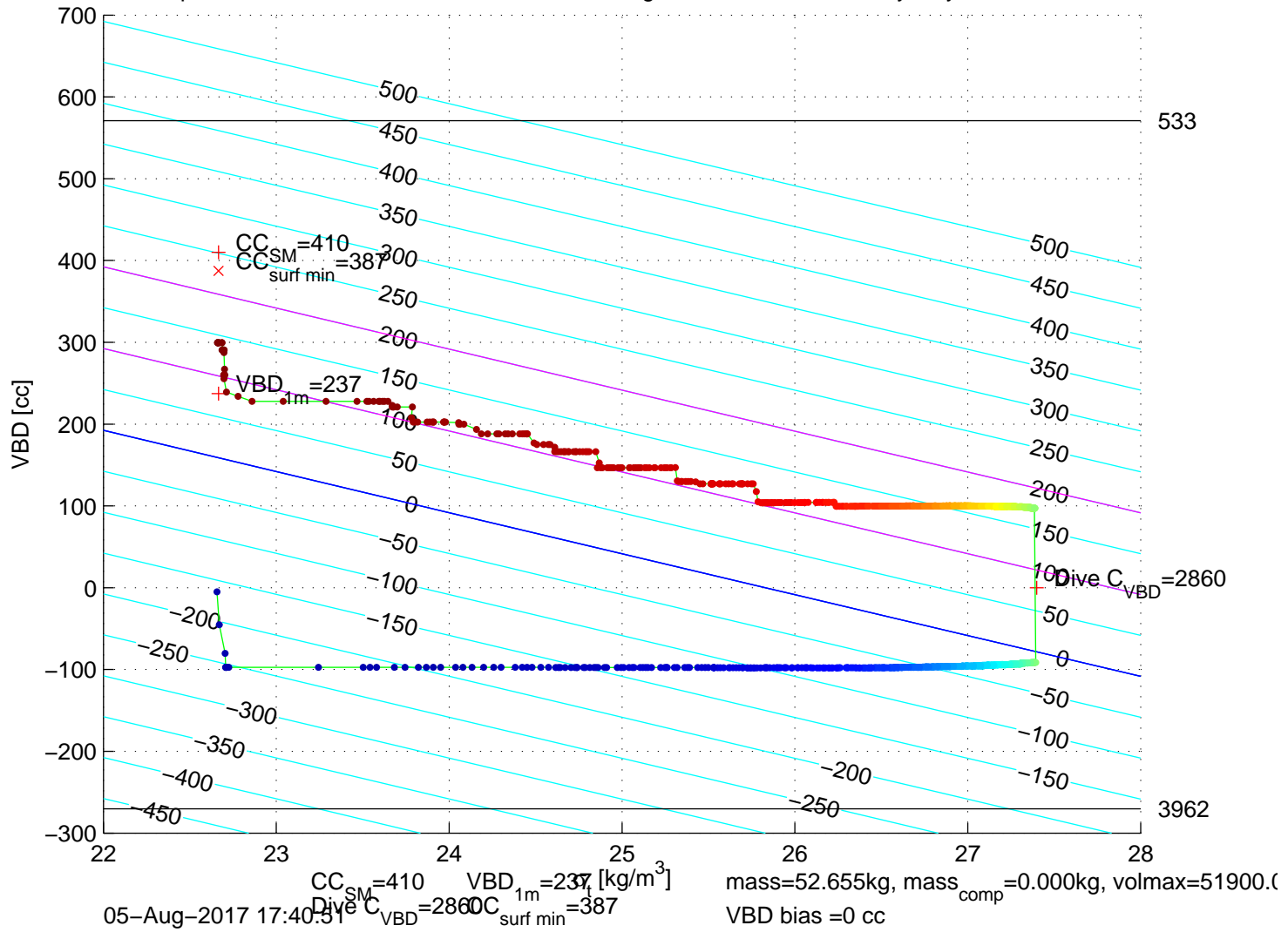
p6350147: SG635 Mission 7 Jul 2017 05–Aug–2017 17:01:21Z – buoyancy contoured
