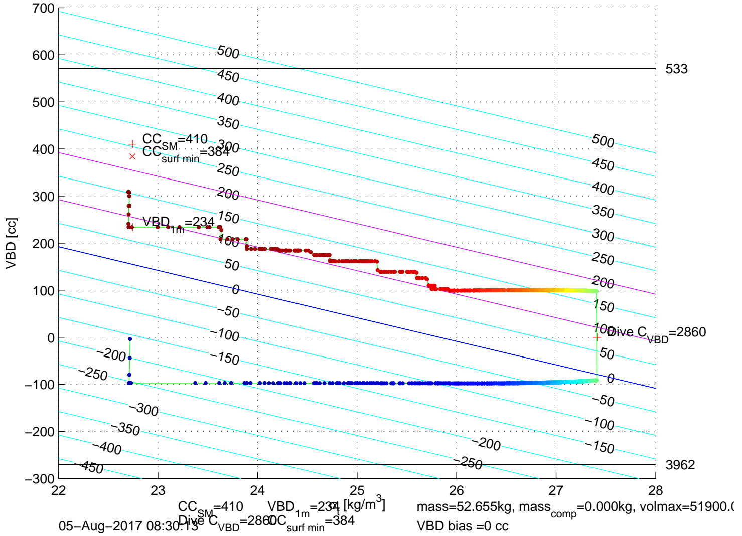
p6350145: SG635 Mission 7 Jul 2017 05–Aug–2017 07:54:57Z – buoyancy contoured
