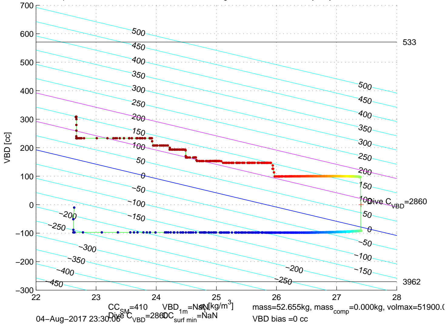
p6350143: SG635 Mission 7 Jul 2017 04-Aug-2017 22:41:34Z – buoyancy contoured
