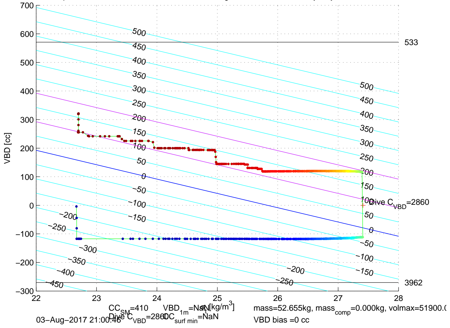
p6350137: SG635 Mission 7 Jul 2017 03–Aug–2017 20:34:17Z – buoyancy contoured
