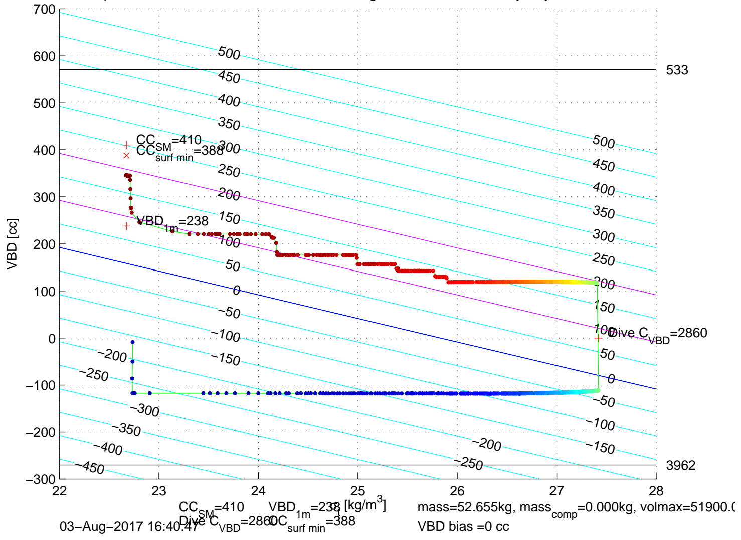
p6350136: SG635 Mission 7 Jul 2017 03–Aug–2017 16:14:20Z – buoyancy contoured
