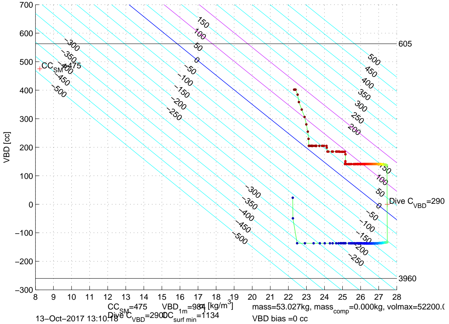
p6300690: SG630 Mission 7 Jul 2017 13–Oct–2017 13:06:25Z – buoyancy contoured
