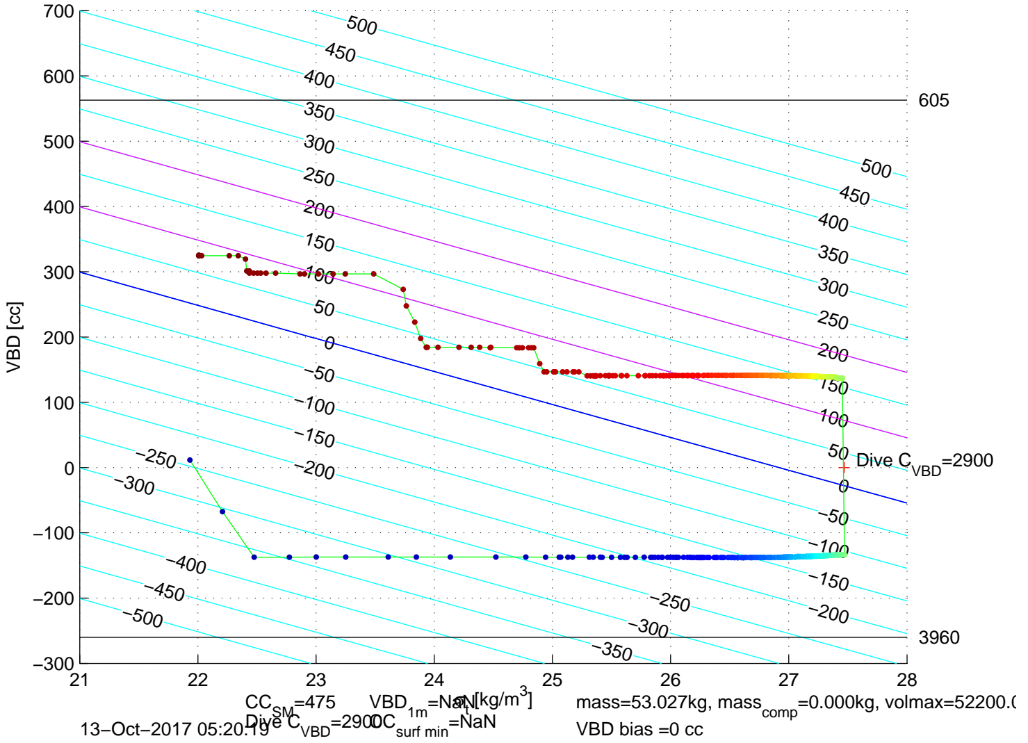
p6300688: SG630 Mission 7 Jul 2017 13-Oct-2017 05:10:25Z – buoyancy contoured
