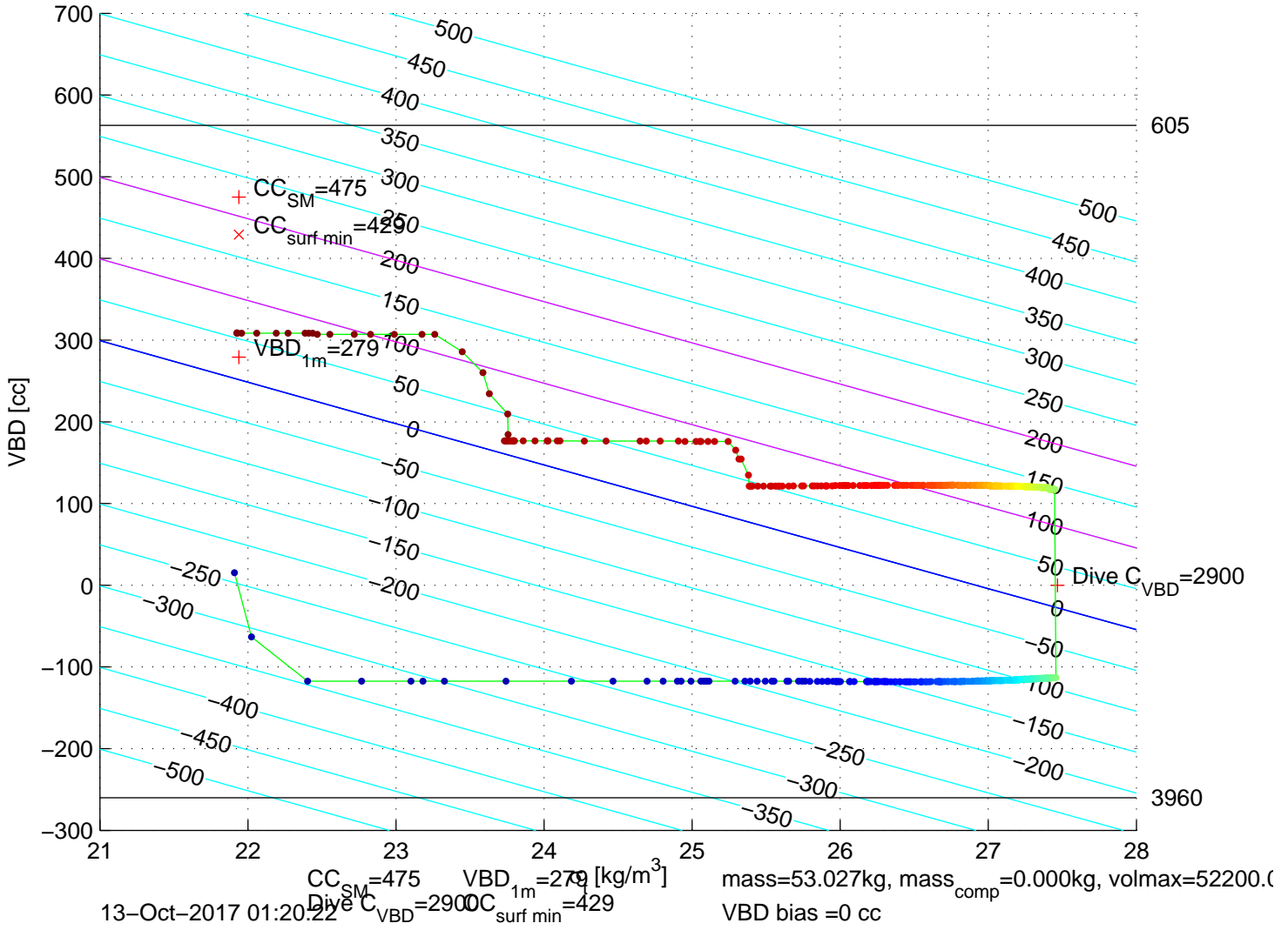
p6300687: SG630 Mission 7 Jul 2017 13-Oct-2017 00:55:34Z – buoyancy contoured
