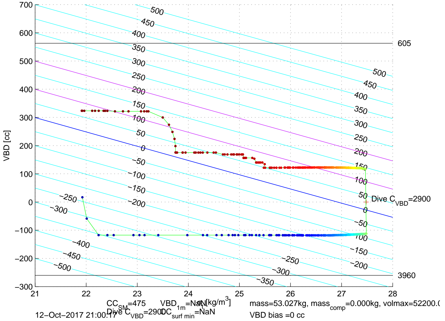
p6300686: SG630 Mission 7 Jul 2017 12–Oct–2017 20:34:18Z – buoyancy contoured
