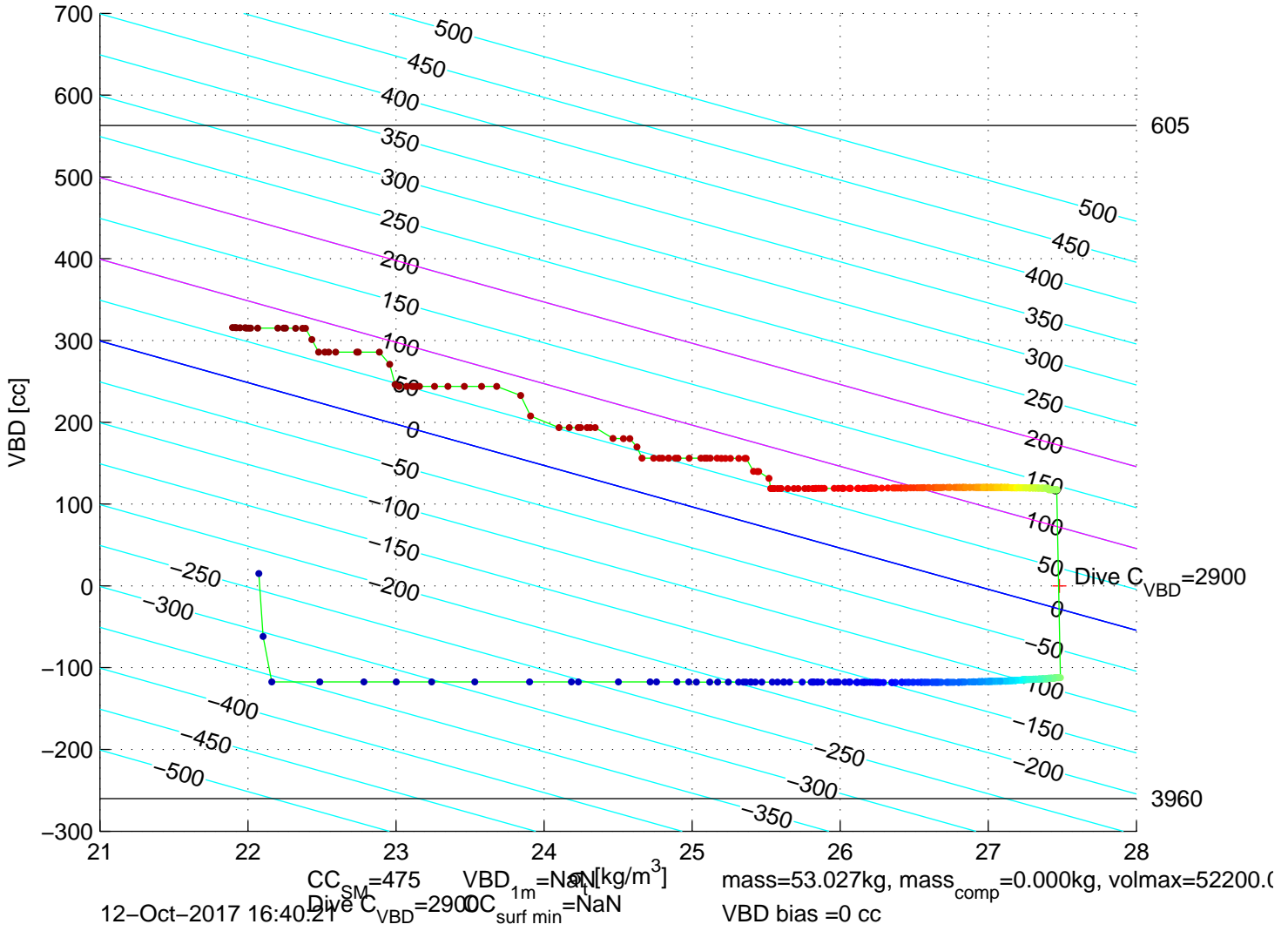
p6300685: SG630 Mission 7 Jul 2017 12–Oct–2017 16:14:25Z – buoyancy contoured
