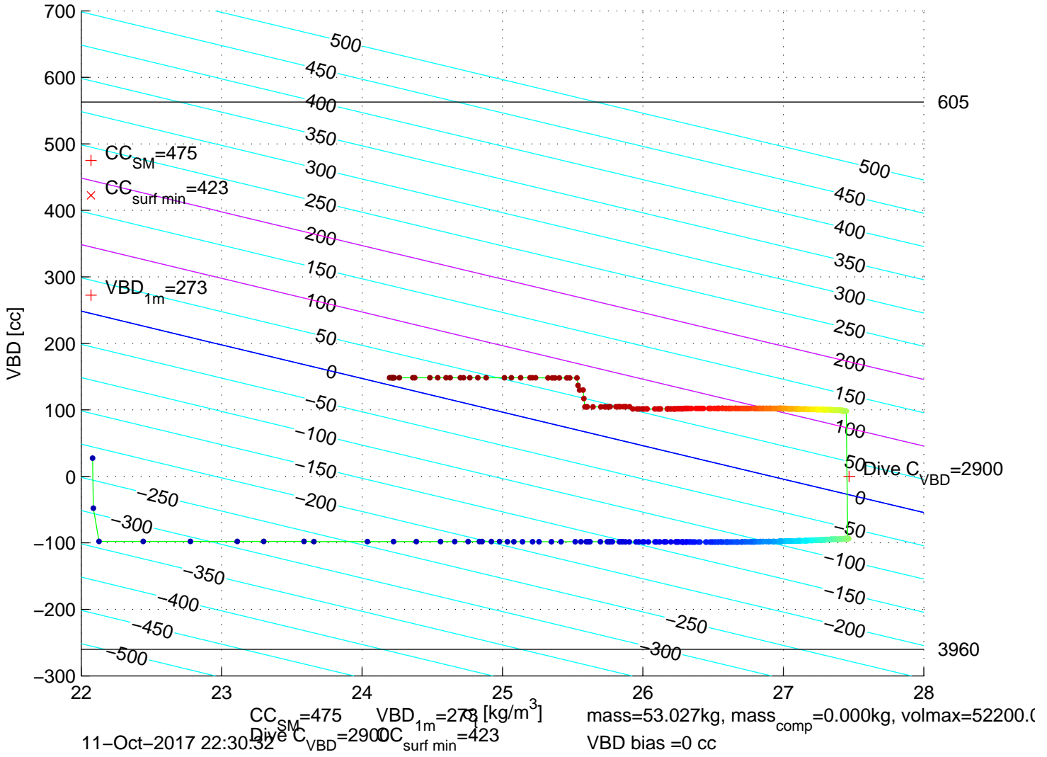
p6300681: SG630 Mission 7 Jul 2017 11–Oct–2017 21:51:30Z – buoyancy contoured
