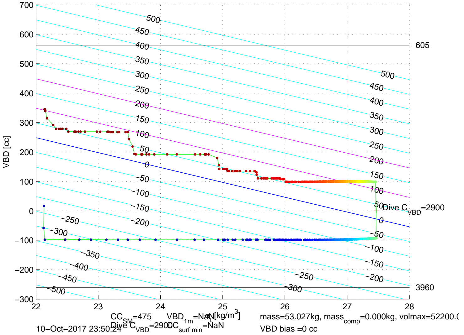
p6300676: SG630 Mission 7 Jul 2017 10–Oct–2017 23:09:00Z – buoyancy contoured
