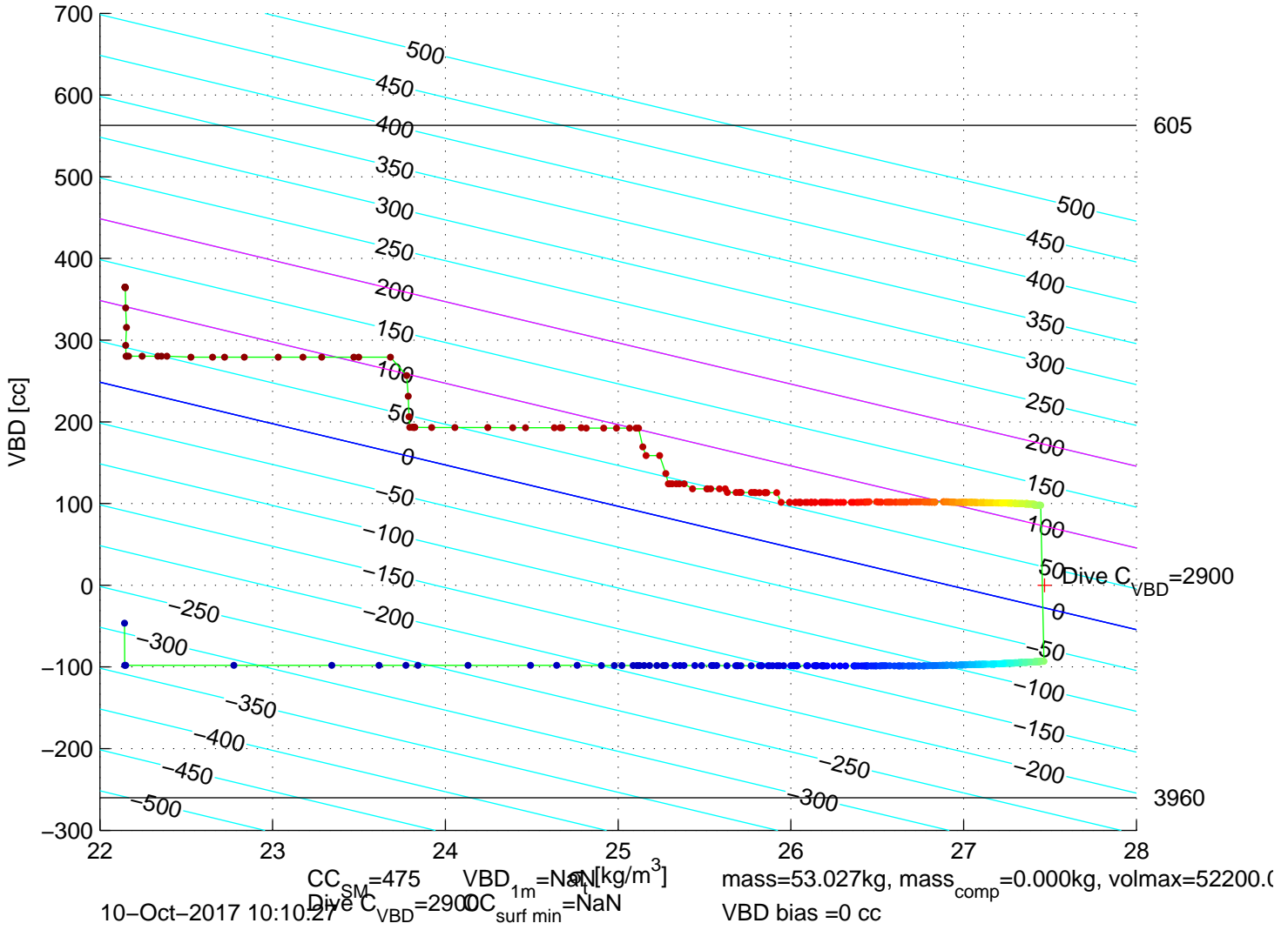
p6300673: SG630 Mission 7 Jul 2017 10–Oct–2017 09:19:16Z – buoyancy contoured
