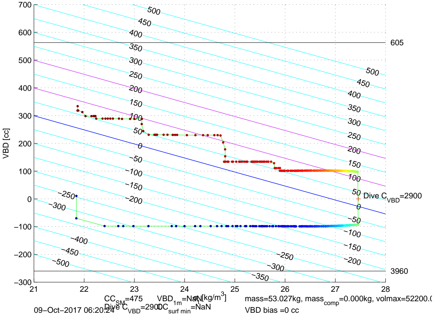
p6300667: SG630 Mission 7 Jul 2017 09–Oct–2017 05:33:01Z – buoyancy contoured
