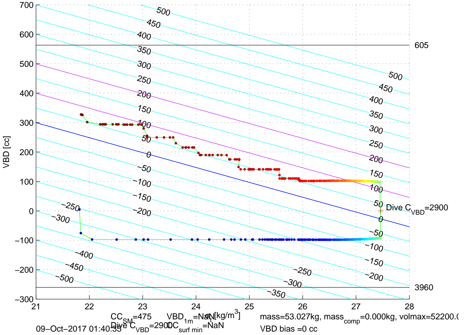
p6300666: SG630 Mission 7 Jul 2017 09–Oct–2017 00:53:53Z – buoyancy contoured
