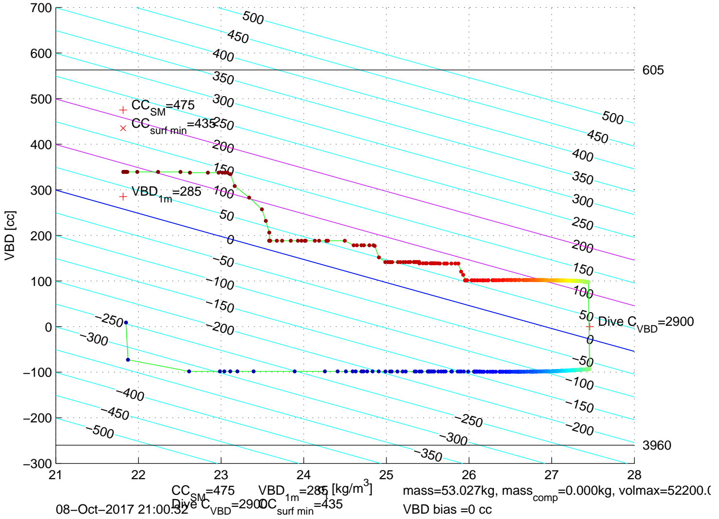
p6300665: SG630 Mission 7 Jul 2017 08–Oct–2017 20:18:08Z – buoyancy contoured
