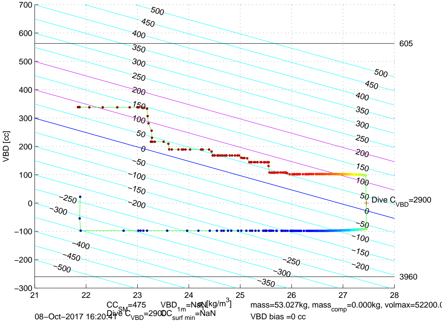
p6300664: SG630 Mission 7 Jul 2017 08–Oct–2017 15:40:03Z – buoyancy contoured
