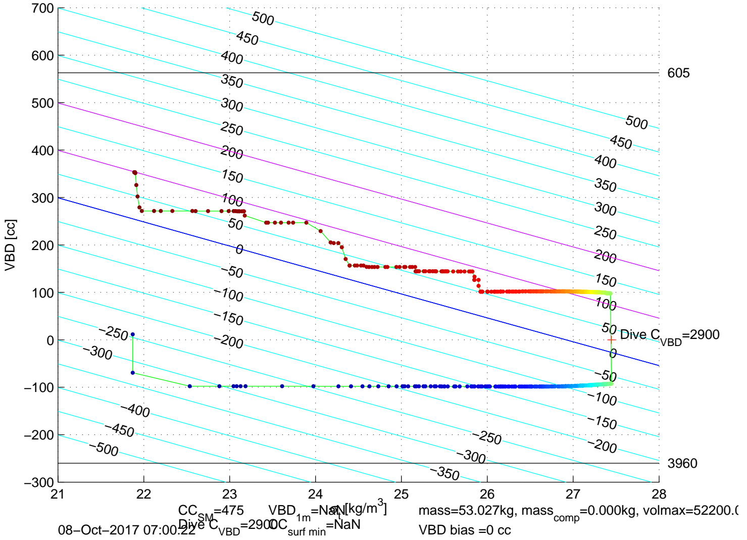
p6300662: SG630 Mission 7 Jul 2017 08–Oct–2017 06:20:45Z – buoyancy contoured
