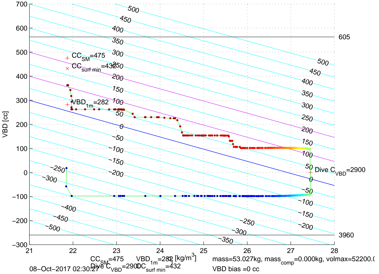
p6300661: SG630 Mission 7 Jul 2017 08–Oct–2017 01:40:17Z – buoyancy contoured
